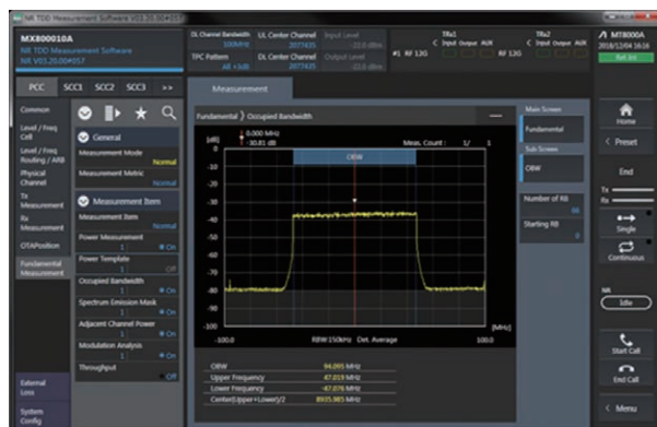
Occupied Bandwidth
