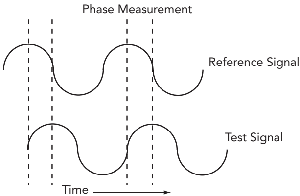
Figure 5. Shown here are signals with a 90-degree phase difference.
