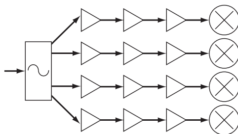
Figure 35. In this four-channel receiver architecture, a single LO is shared between four down converters. Amplifier chains are used to ensure channel-to-channel isolation. More or fewer amplifiers can be used and, in some circumstances, the engineer might even opt to use isolators or filters instead.
