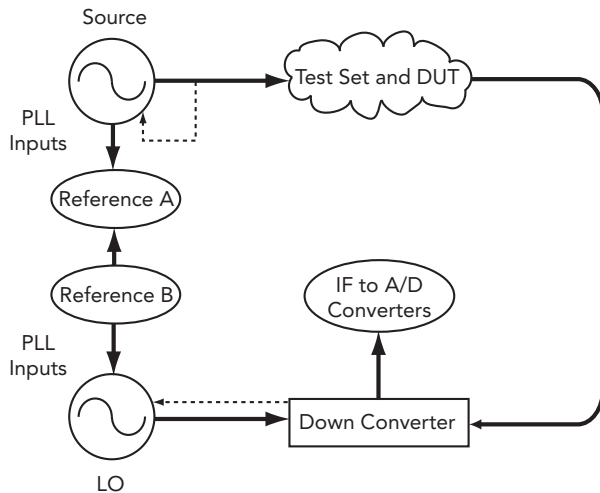
Figure 24C. A follower architecture is shown here. In this case, the LO is locked to the IF. Since the loop tries to keep the IF clean, noise on the source is transferred, in a canceling fashion, to the LO.
