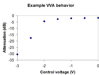
Figure 26. An example response curve of a commercial voltage-variable-attenuator is illustrated in this graphic.
